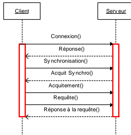
Figure 14 : Communication TCP/IP
