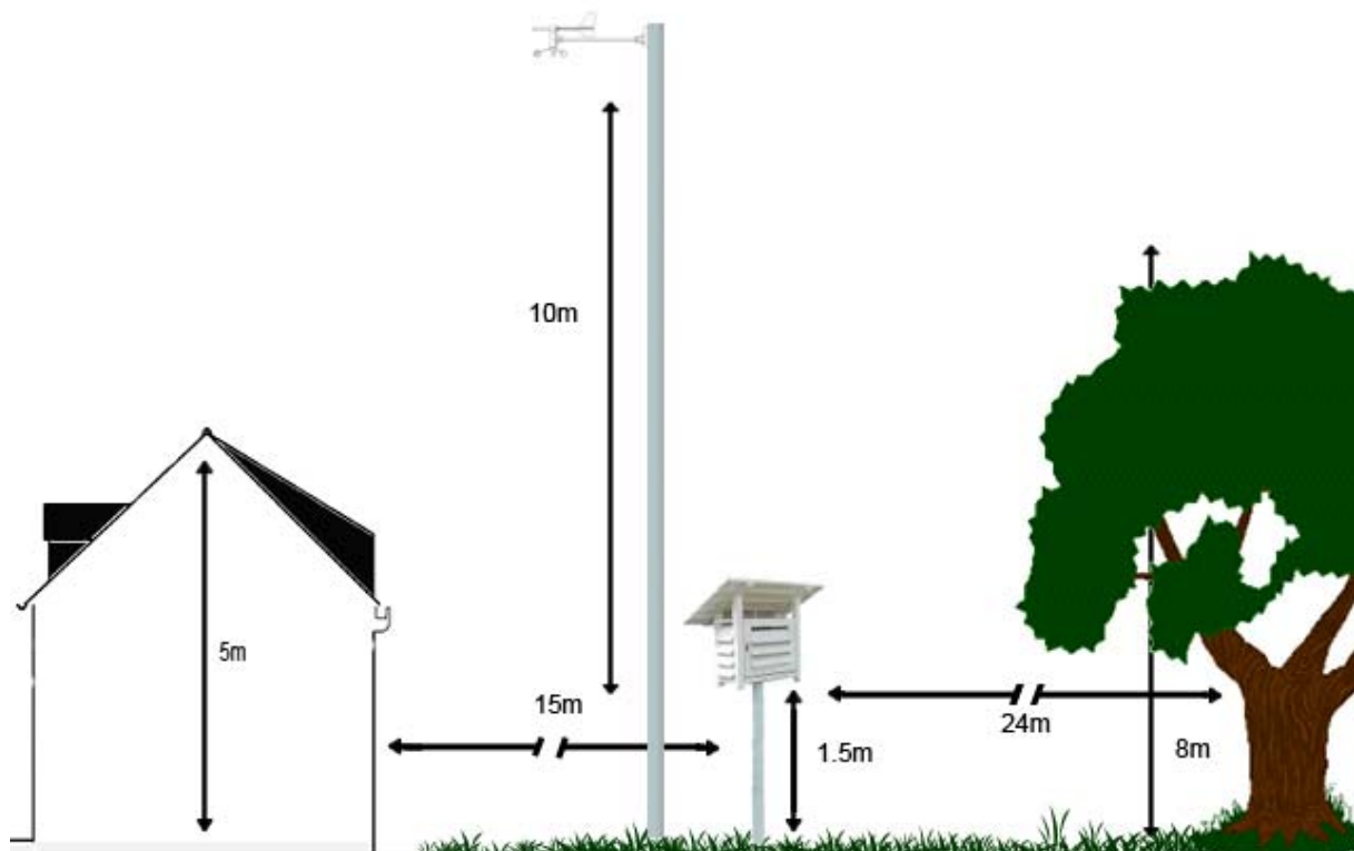
Figure 8: Implantation de la station
